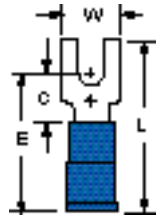
MV14-6FB Stud Size: 6 Wire Range: 16-14
