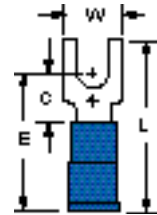
MV14-8FB Stud Size: 8 Wire Range: 16-14
