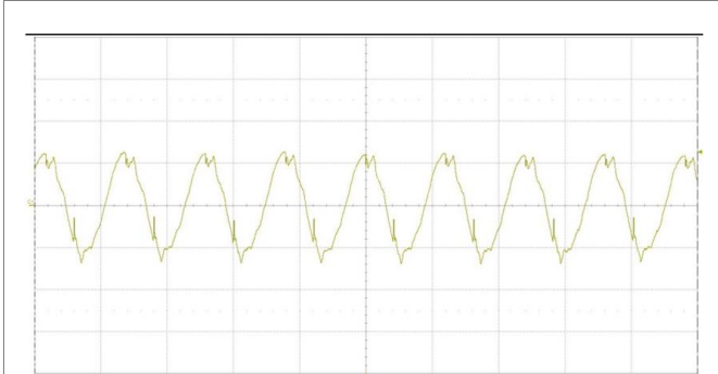
Output voltage ripple at: T_{P1} = +25^{\circ}\text{C} , V_I = 48\text{ V} , I_O = 4.2\text{ A} resistive load. Trace: output voltage (20 mV/div.). Time scale: (2 \mu\text{s} /div.). 20 MHz bandwidth.
