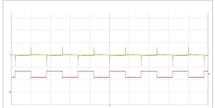
Output voltage response to load current step- change (2.1-3.15-2.1 A) at: T_{P1} = +25^{\circ}\text{C} , V_I = 48\text{ V} . Top trace: output voltage (500 mV/div.). Bottom trace: load current (2 A/div.). Time scale: (10 ms/div.).
