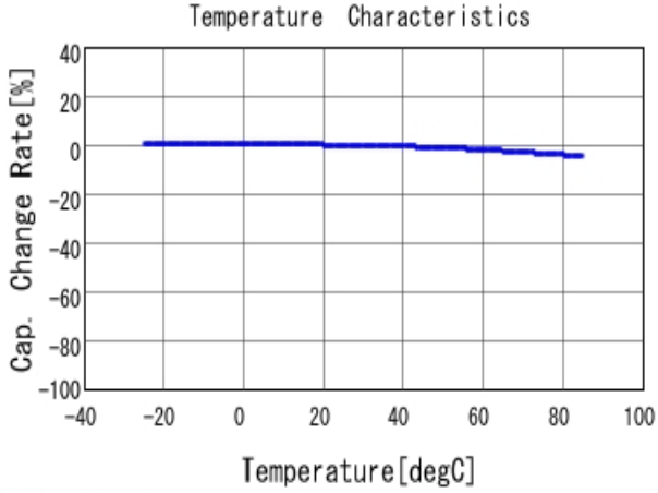
■ GRM188B31H104KA92 C-Temp. capchange, DC0.0V, AC1.0V r m
