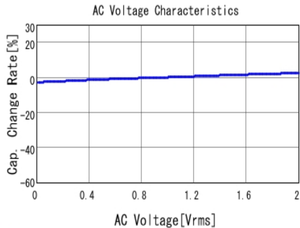
■ GRM188B31H104KA92 C-AC Voltage capchange, DCOV, 20.0d
