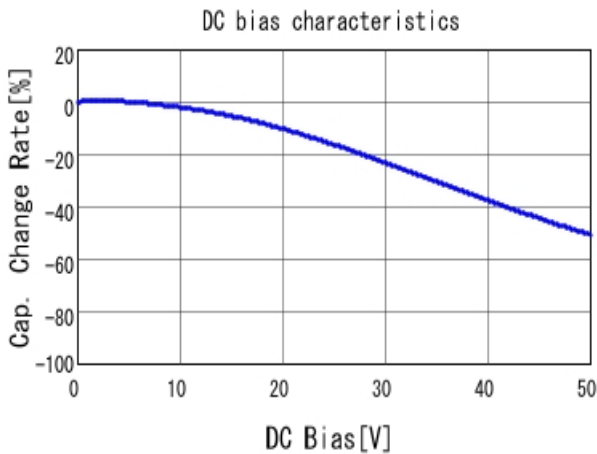
■ GRM188B31H104KA92 C-DC bias capchange, 20.0degC, AC1.
