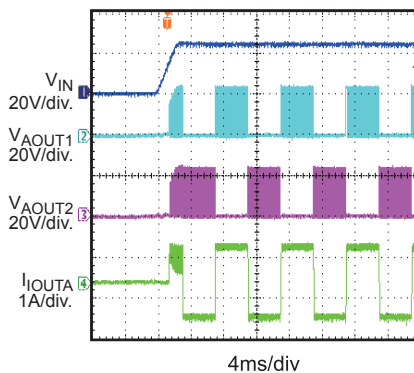
Power Ramp Up-Full Step I_{OUT}=1A
