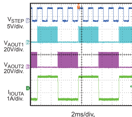
Steady State-Full Step I_{OUT}=1A
