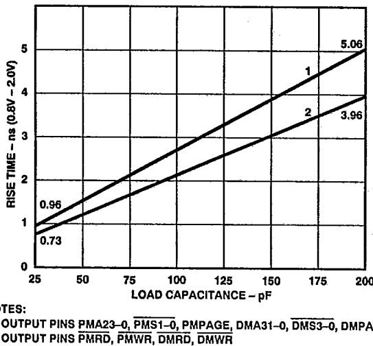
Figure 17. Typical Output Rise Time vs. Load Capacitance (at Maximum Case Temperature)
