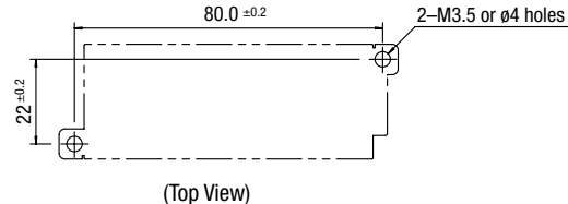
(Panel Mounting Hole Layout)
