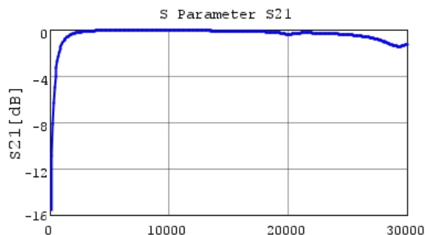
GRM0225C1H2R7CA03 S21 DCOV, 25degC
