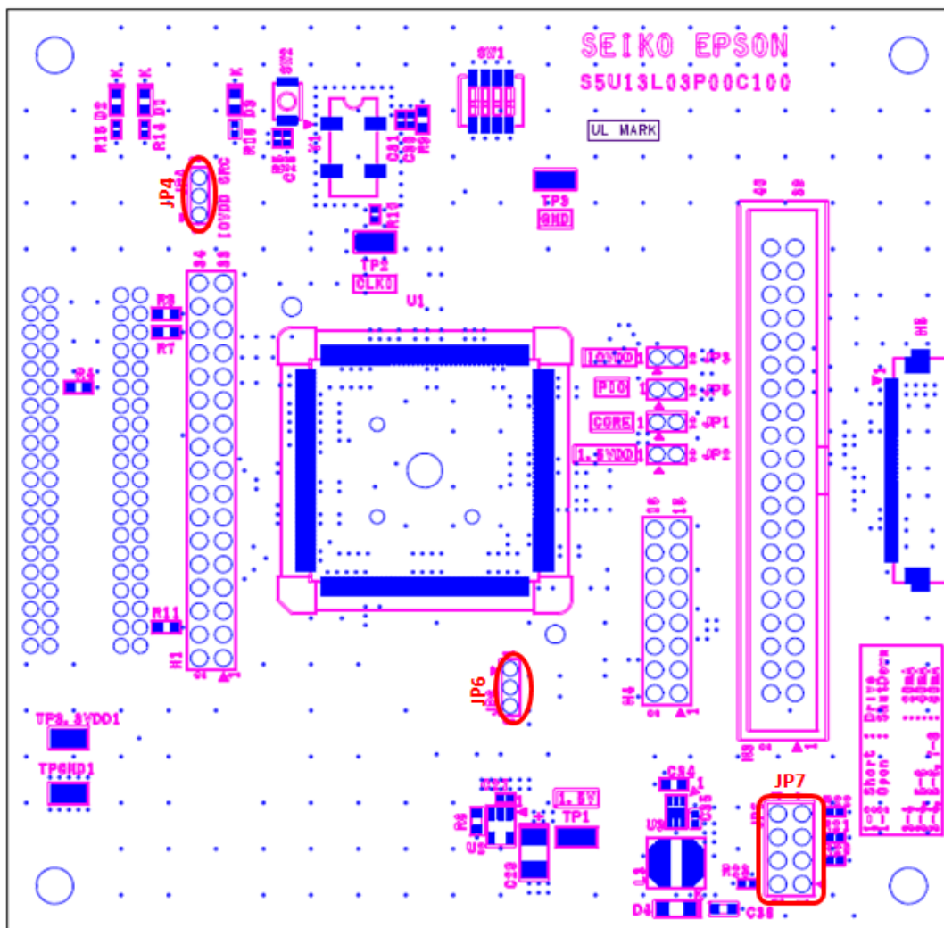
Figure 3-3: Configuration Jumper Location (JP4, JP6, JP7)
