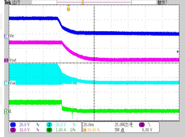
I_{out} = 0.6A
