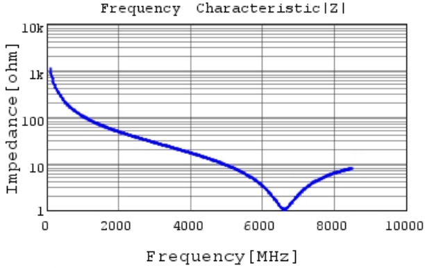
GCM1555C1H1R5BA16 |Z| DC0V, 25degC
