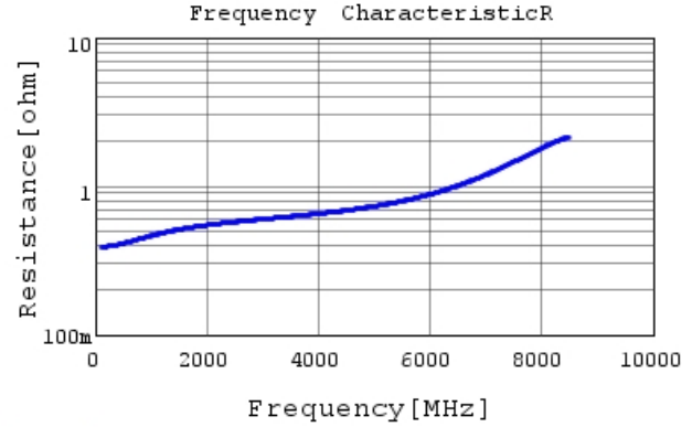
GCM1555C1H1R5BA16 R DC0V, 25degC
