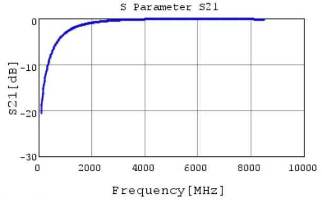
GCM1555C1H1R5BA16 S21 DCOV, 25degC
