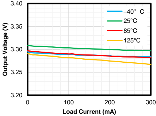
Figure 7. Load Regulation
