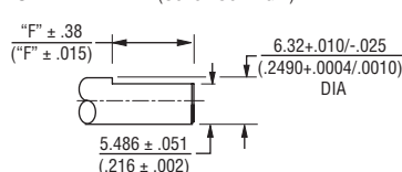
SHAFT TYPE "H" (USES BUSHING A)
