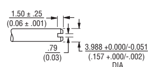
SHAFT TYPE "T" (USES BUSHING U)
