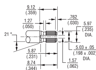
SHAFT TYPE "Y" (USES BUSHING A)
