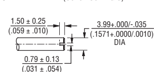
SHAFT TYPE "V" (USES BUSHING U)
