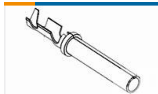
TE Part #776493-1 SOC, SF, SIZE 16, 18-20 AWG, AU/SN
