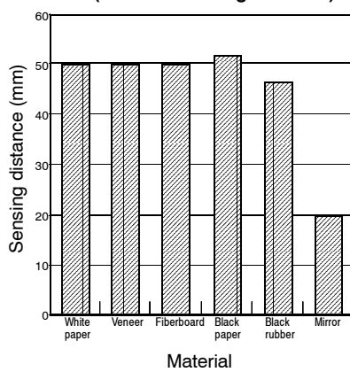
E3G-L1 (at 50 mm Setting Distance)
