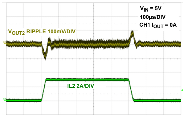
FIGURE 16. LOAD TRANSIENT CHANNEL 2
