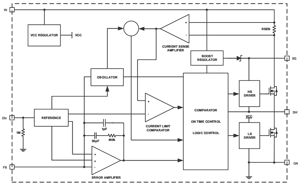
MP2359DJ-LF-Z Block Diagram
