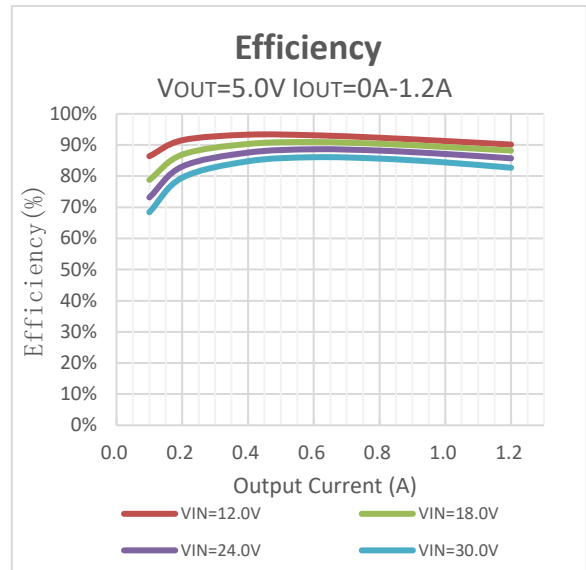
Efficiency V_{OUT}=5V
