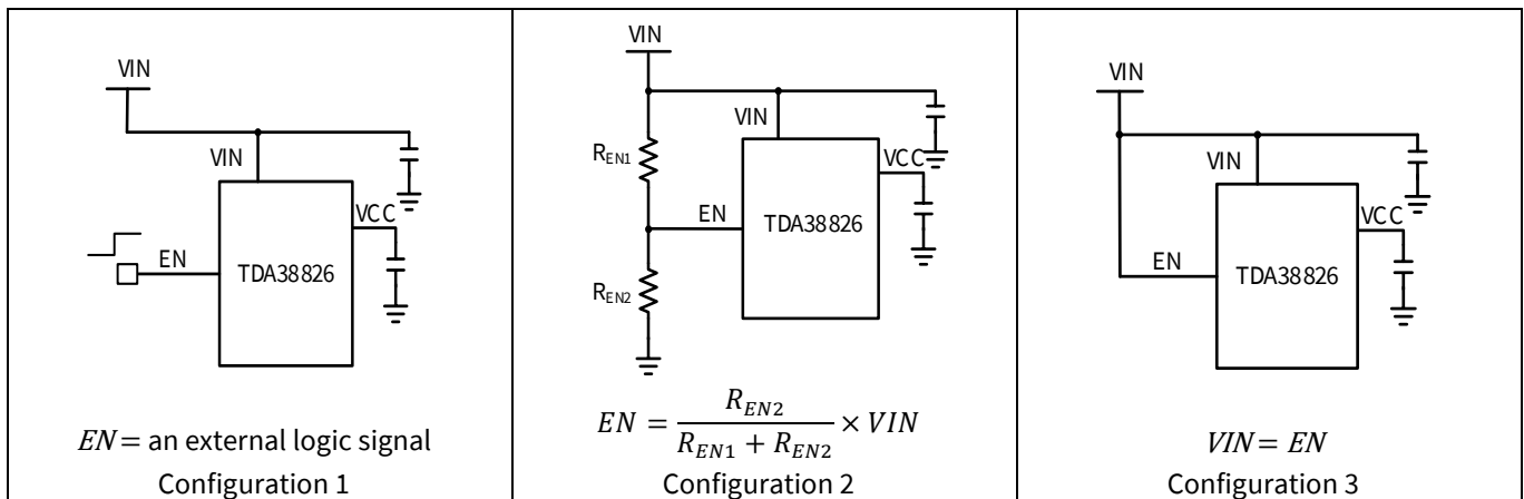
Figure 8 Enable Configurations
