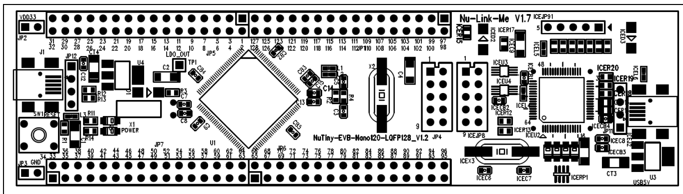
Figure 2-2 NuTiny-SDK-NANO120 PCB Placement
