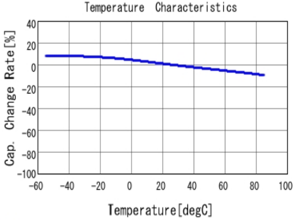
■ GRM155R61H104KE19 C-Temp. capchange, DC0.0V, AC1.0V rm
