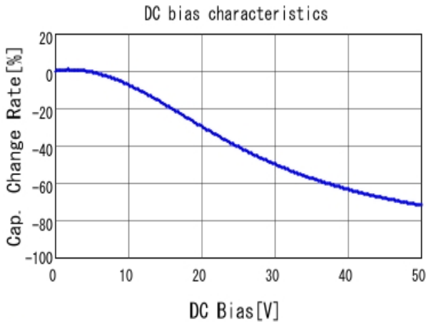
■ GRM155R61H104KE19 C-DC bias capchange, 25.0degC, AC1.
