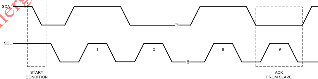
Figure 8. I 2 C acknowledge.
