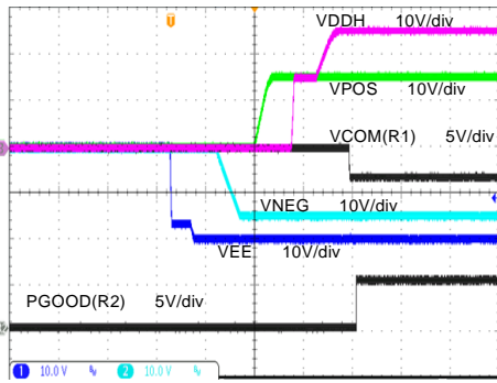
Default Power-up Sequence
