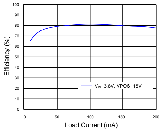
VPOS Positive LDO Efficiency
