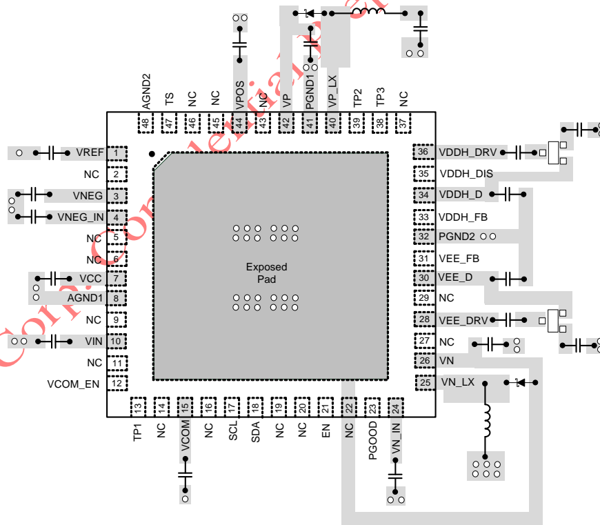
Figure 9. Conceptual PCB Layout Guide
