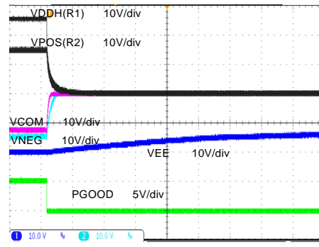
Default Power-off Sequence
