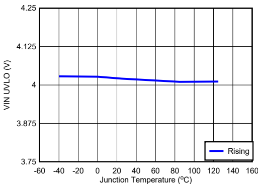
Figure 6-7. V_{IN} UVLO
