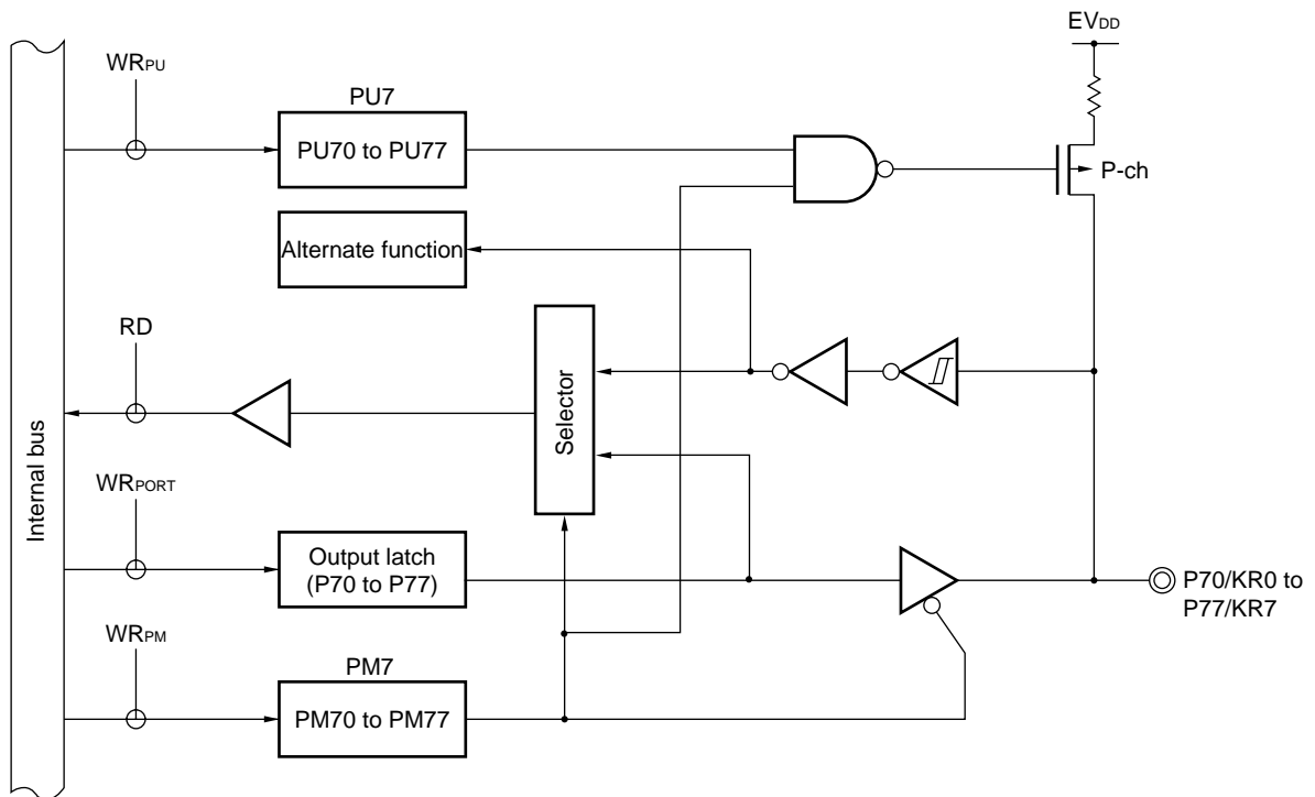
Figure 4-17. Block Diagram of P70 to P77
