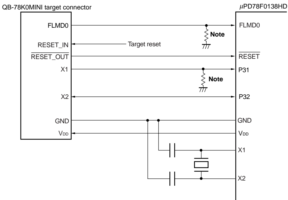
Figure 27-2. Connection Example of QB-78K0MINI and μPD78F0138HD (When P31 and P32 Are Used)
