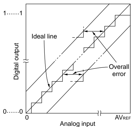
Figure 12-13. Overall Error
