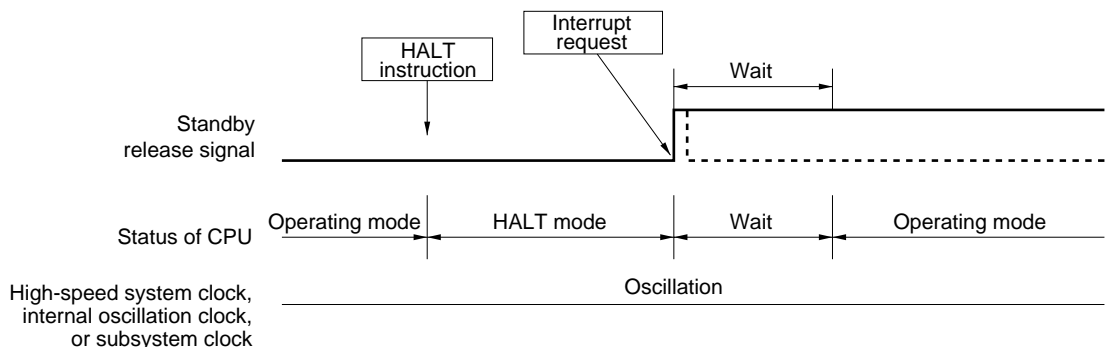
Figure 19-3. HALT Mode Release by Interrupt Request Generation
