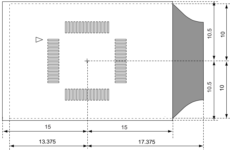
Figure B-1. Restricted Areas on Target System (64-Pin GB Package)
