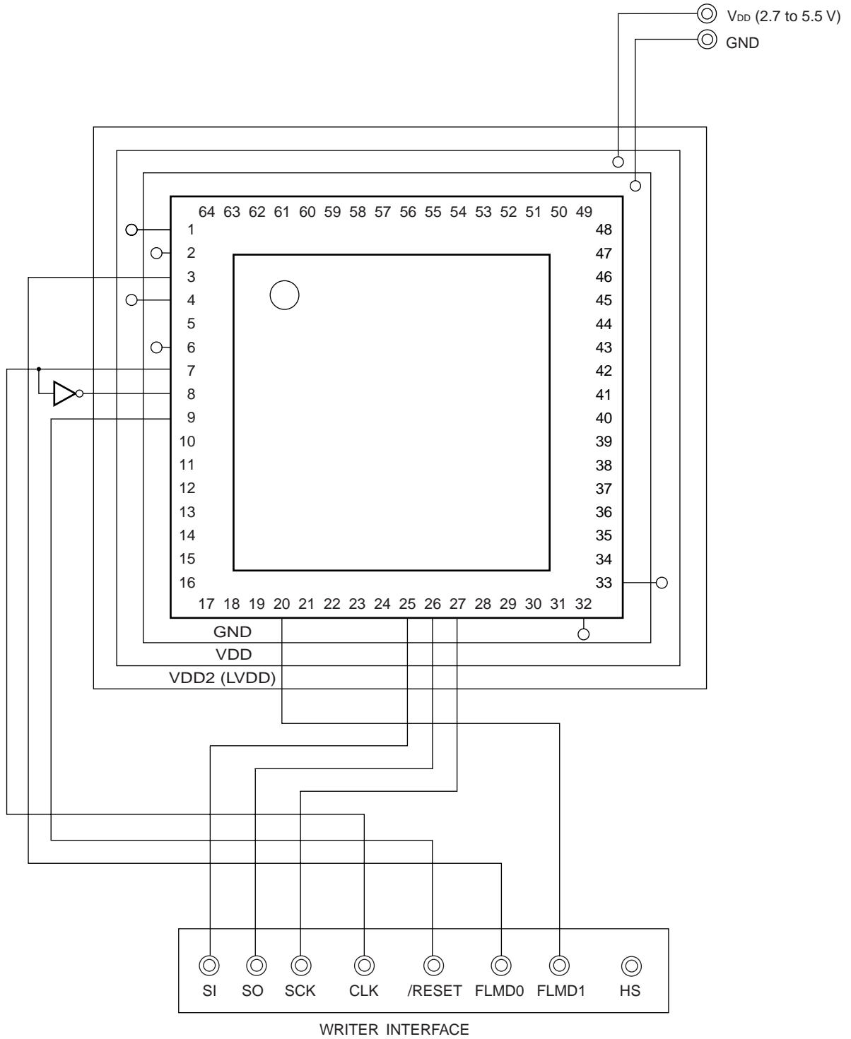
Figure 26-3. Example of Wiring Adapter for Flash Memory Writing in 3-Wire Serial I/O (CS110) Mode
