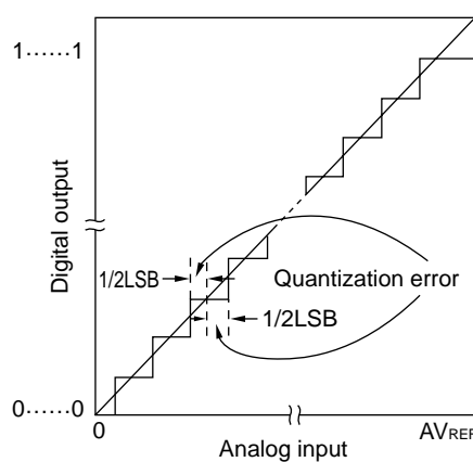
Figure 12-14. Quantization Error
