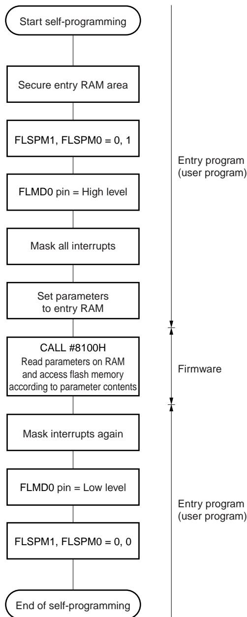
Figure 26-18. Self-Programming Procedure
