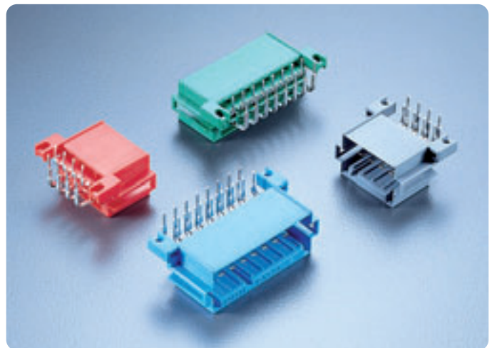
DCS right angled pin-headers 8 & 16 ways
