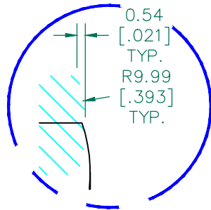
DETAIL "A" RADIUS SCALE=3:1
