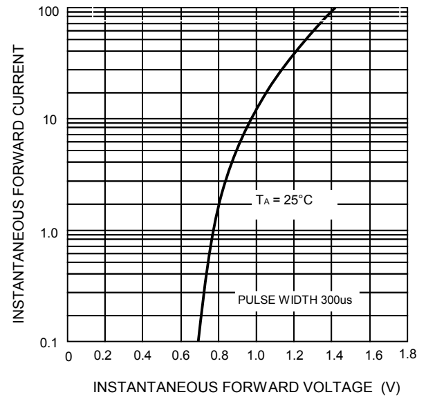
FIG.2-TYPICAL FORWARD CHARACTERISTICS
