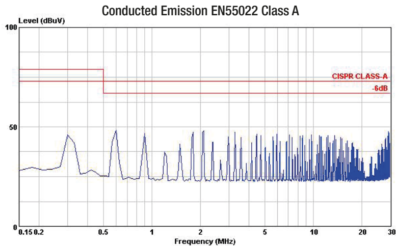
EMI Filtering according to EN55022/11 Class A and EN50121-1 (110Vin)
