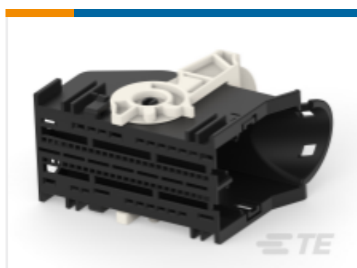
TE Part #2177472-1 73POS, MIXED,REC HSG,ASSY,BK
