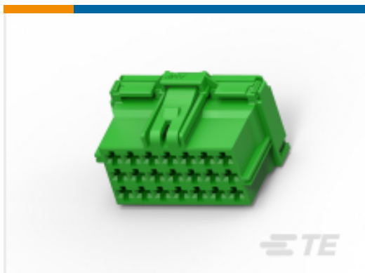
TE Part #1452299-1 AMP Unsealed Connector Housing
