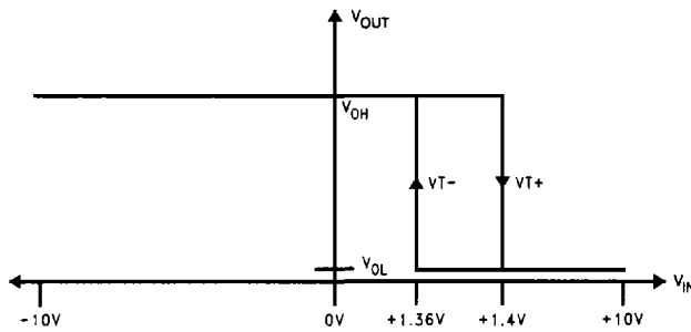
FIGURE 7. Receiver Threshold Voltage Transfer Curve (VTC)
