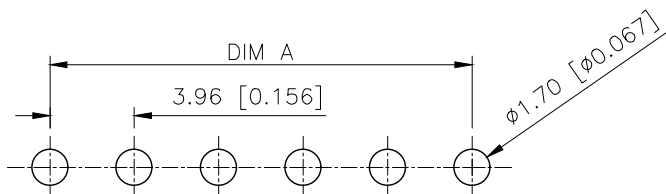
PCB LAYOUT
