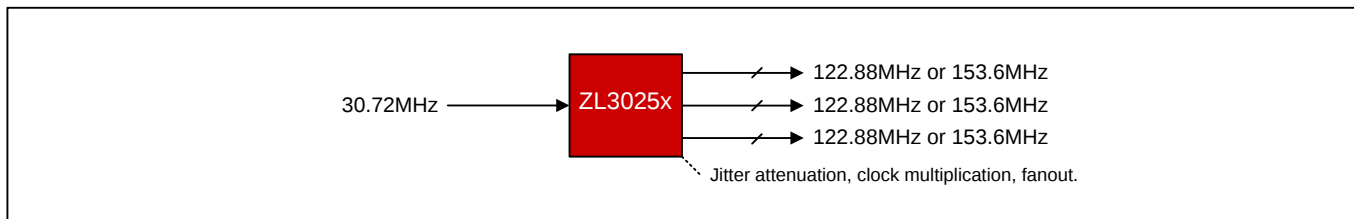
Figure 3 – Wireless Base Station Jitter Filtering and Frequency Conversion Application
