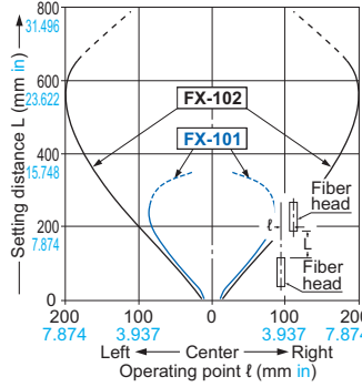
FD-G6X Reflective type
