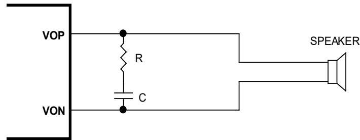
Figure 32: Class-D Output RC Snubber Circuit
