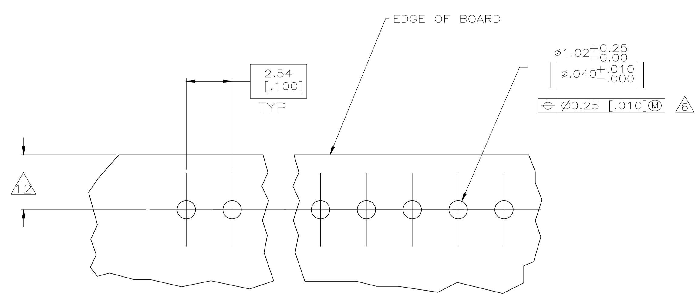
RECOMMENDED MOUNTING HOLE PATTERN \Delta FOR 1.60 [0.063] THICK P.C. BOARD
