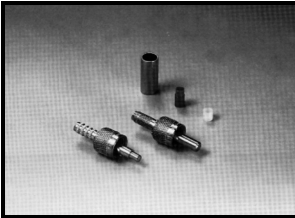
905/906-150 Series Stainless Steel SMA Connectors
