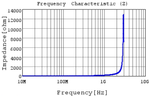
LQP03TN24NH02 |Z|
