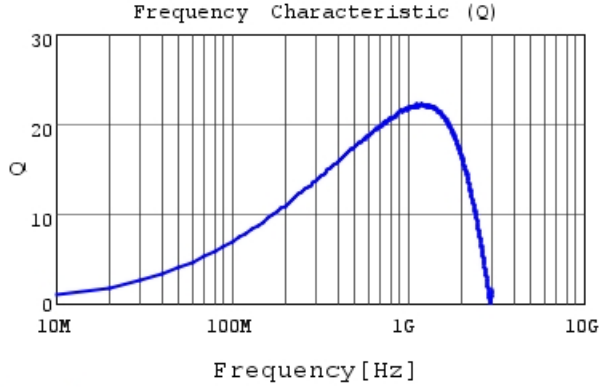
LQP03TN24NH02 Q
