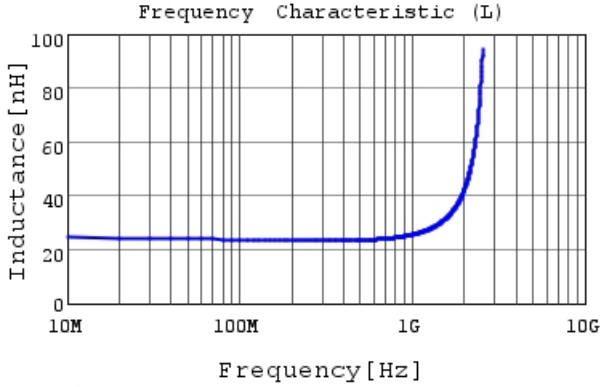
LQP03TN24NH02 L
