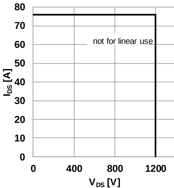
Figure 1 Safe operating area (SOA) (V_{GS} = 0/18V, T_c = 25^\circ C, T_j < 175^\circ C)
