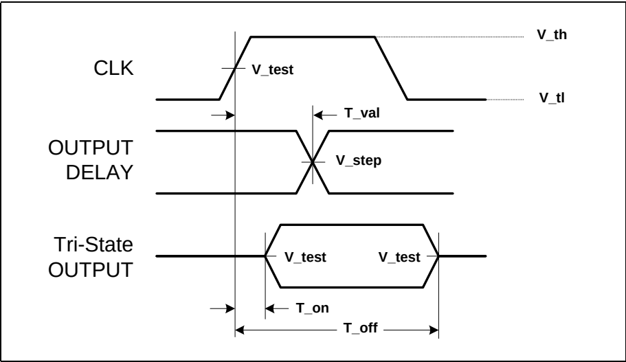
Figure 21. Output Timing Measurement Conditions
