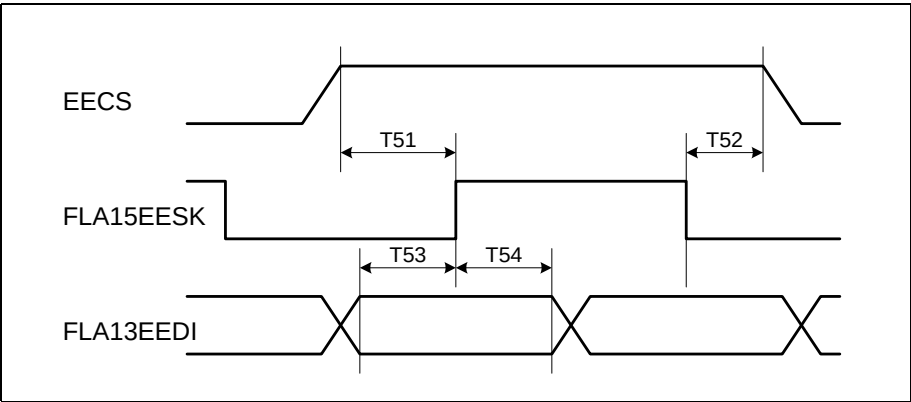
Figure 25. EEPROM Timings
