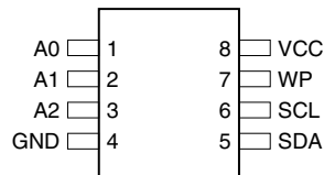
8-lead TSSOP
