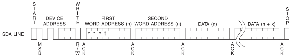
Figure 7-3. Page Write
