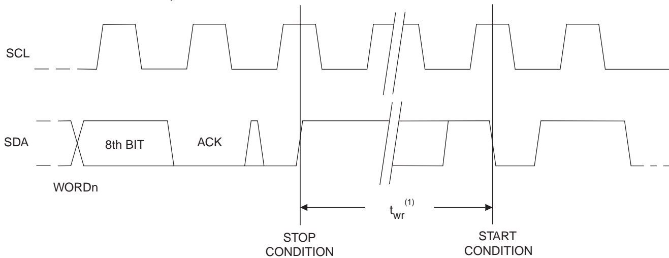
Figure 4-3. Write Cycle Timing
