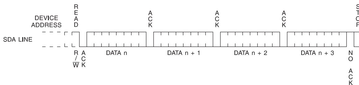
Figure 7-6. Sequential Read
