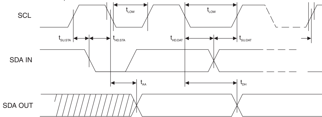
Figure 4-2. Bus Timing
