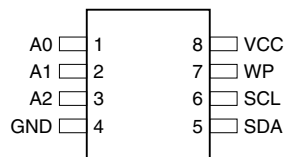
8-lead TSSOP
