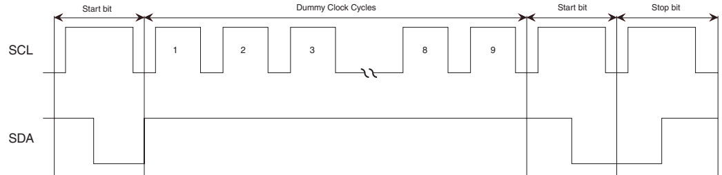
Figure 4-1. Software Reset
