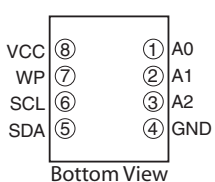
8-ball dBGAA2
