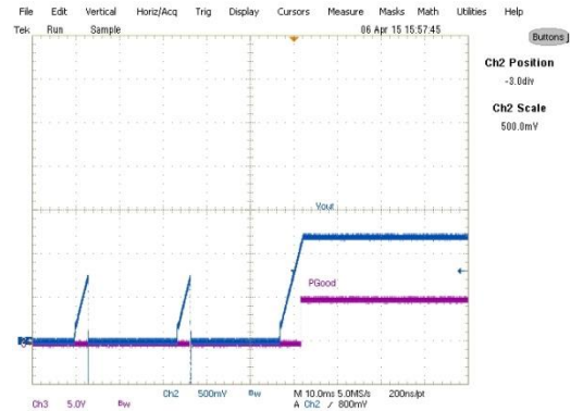
Fig. 9: Short-circuit recovery (Hiccup) at 25A load Ch 2 :V out , Ch 3 :P Good
