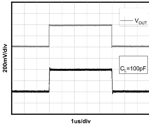
Figure 6. Small-Signal Step Response( V_S=5V )
