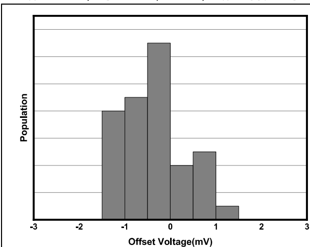
Figure 2. Offset Voltage Production Distribution
