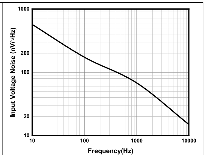
Figure 3. Input Voltage Noise Spectral Density
