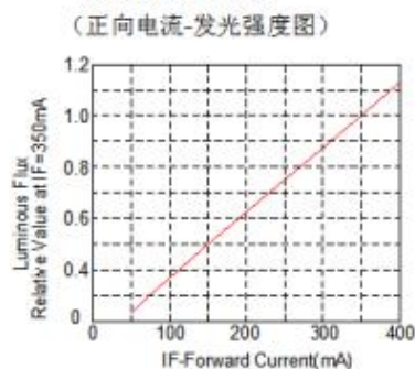
Forward current - luminous intensity curve (正向电流-发光强度图)
