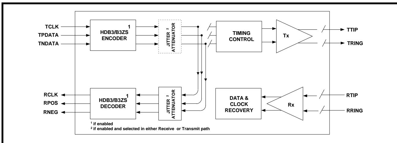
FIGURE 27. DIGITAL LOOPBACK
