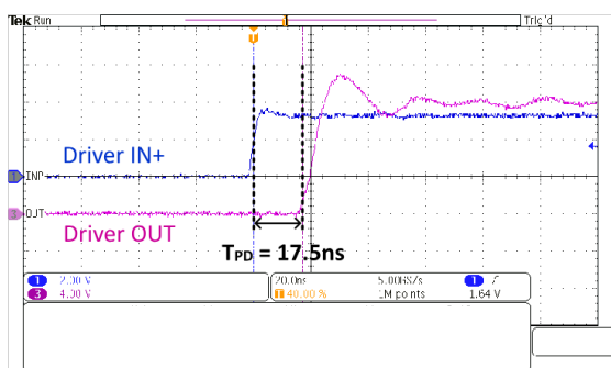
Figure 7-3. UCC27614-Q1 Rising (Turn-On) Propagation Delay
