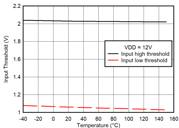
Figure 5-15. Input Threshold vs Temperature
