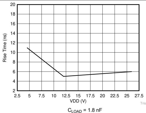
Figure 5-6. Output Rise Time vs VDD
