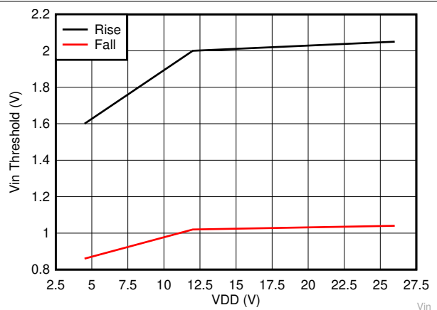
Figure 5-14. Input Threshold vs VDD
