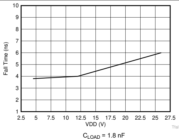
Figure 5-7. Output Fall Time vs VDD
