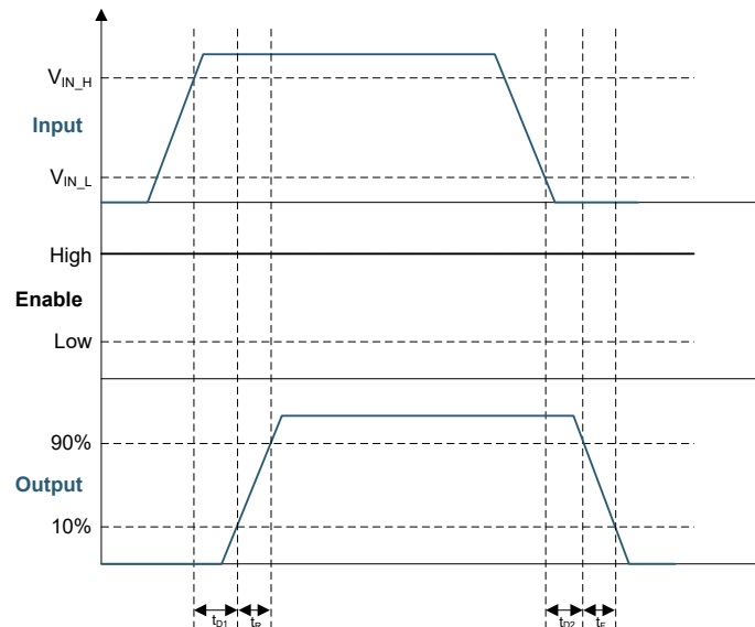
Figure 5-1. Single Input Version, I_{IN} = \text{PWM}
