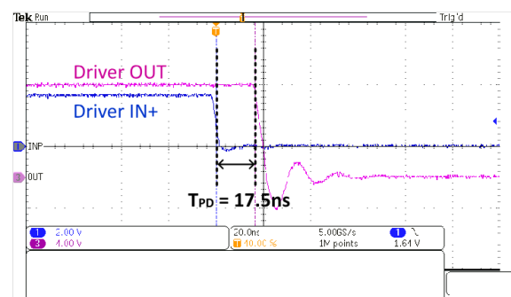
Figure 7-4. UCC27614-Q1 Falling (Turn-Off) Propagation Delay
