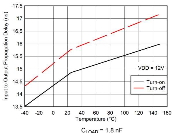
Figure 5-11. Propagation Delay vs Temperature
