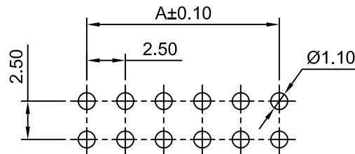
P.C.B LAYOUT TOLERANCE:±0.05
