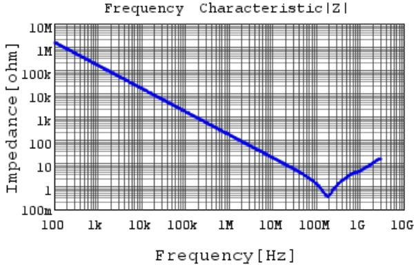
GRM31BR73A102KW01 |Z| DCOV, 25degC
