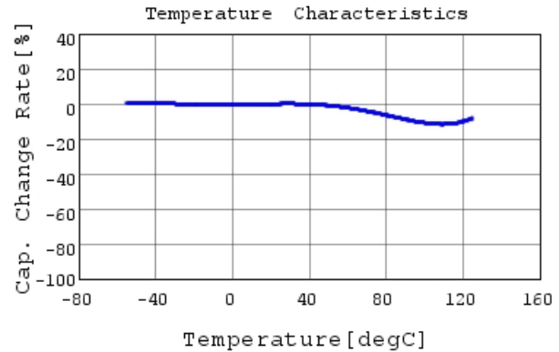
GRM31BR73A102KW01 C-Temp. capchange, DCOV, 1
