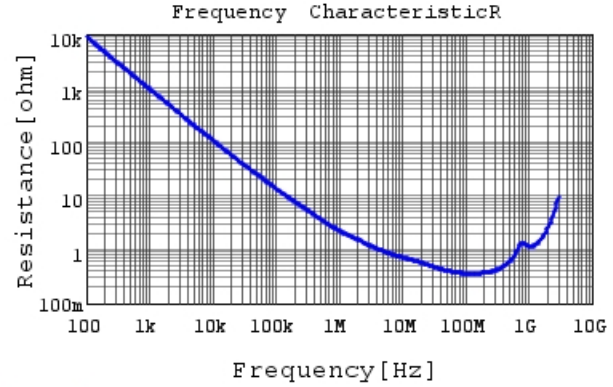
GRM31BR73A102KW01 R DCOV, 25degC
