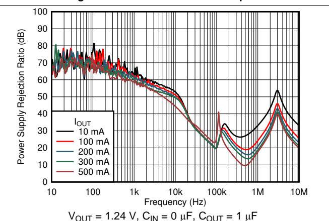
Figure 18. PSRR vs Frequency and I_{OUT}
