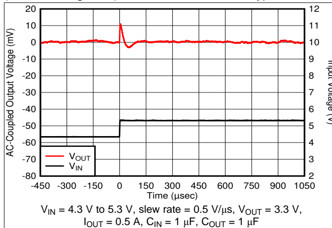
Figure 31. Line Transient
