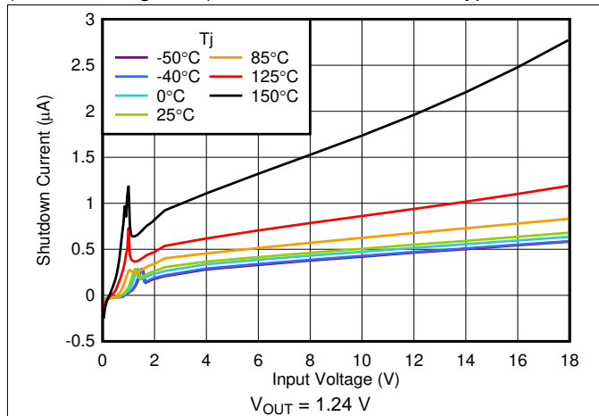
Figure 13. Shutdown Current vs V_{IN}
