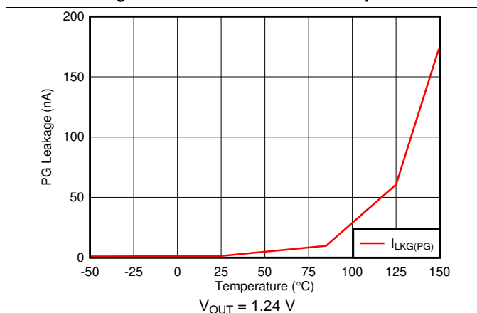
Figure 17. PG Leakage Current vs Temperature
