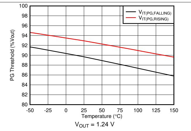
Figure 16. PG Thresholds vs Temperature
