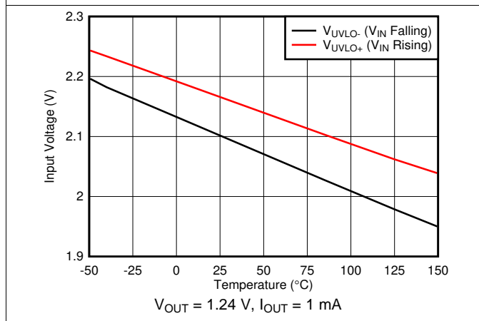
Figure 15. UVLO Thresholds vs Temperature
