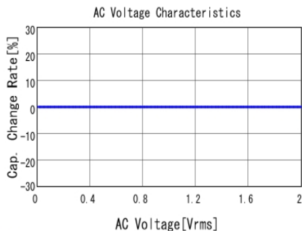
■ GRM0332C1H110JA01 C-AC Voltage capchange, DC0V, 20.0d
