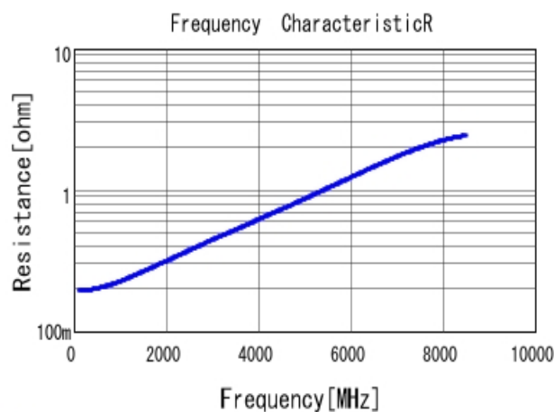
■ GRM0332C1H110JA01 R DC0V, 20degC
