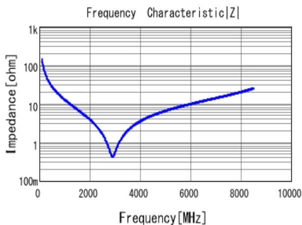
■ GRM0332C1H110JA01 |Z| DC0V, 20degC
