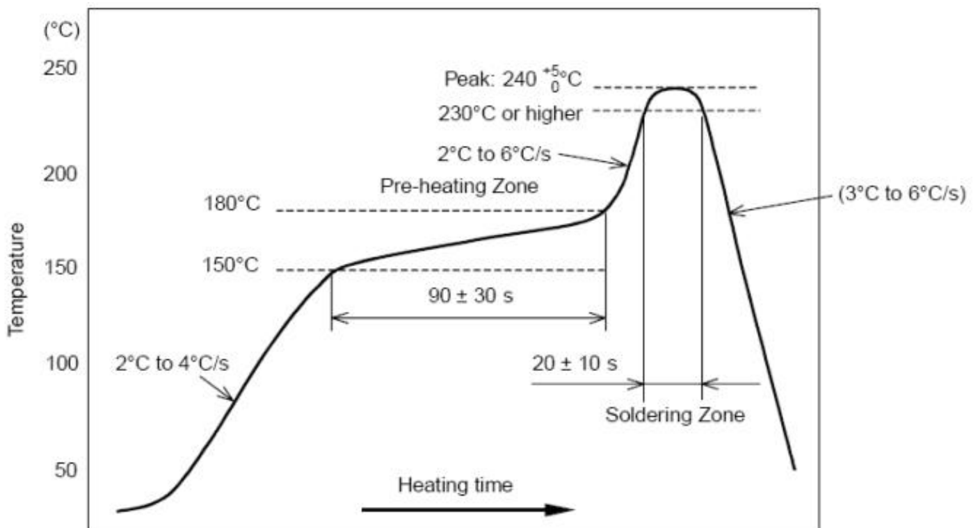
部件的焊接耐热性温度曲线 (焊接点)
