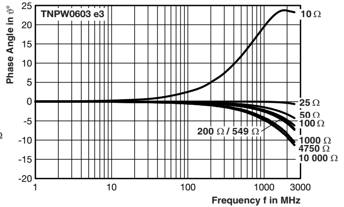
HF Performance (1)
