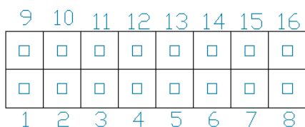
Figure 15: GPO Header
